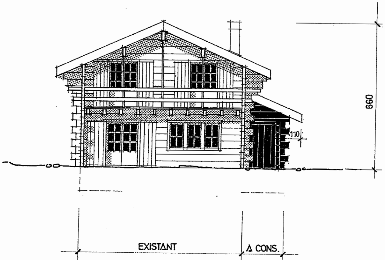
FACADE SUD
